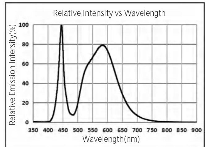
CCT : 4000K (70 CRI)
