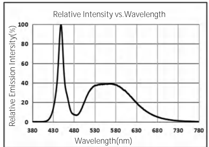
CCT : 5700K (70 CRI)
