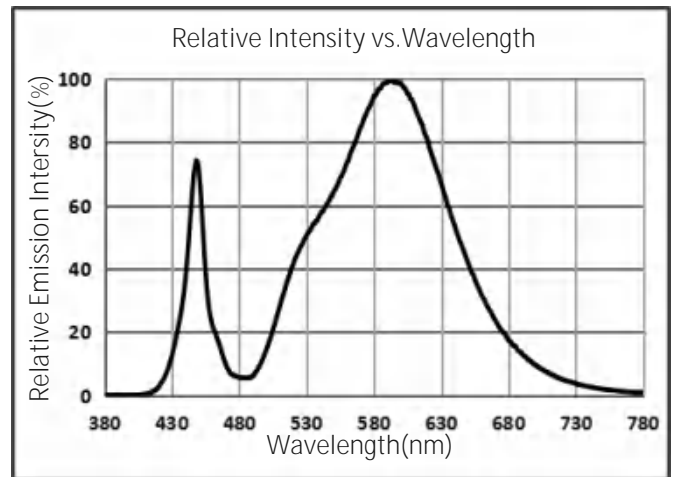
CCT : 3000K (70 CRI)
