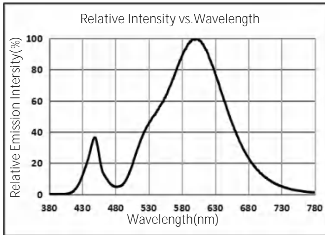
CCT : 2700K (70 CRI)
