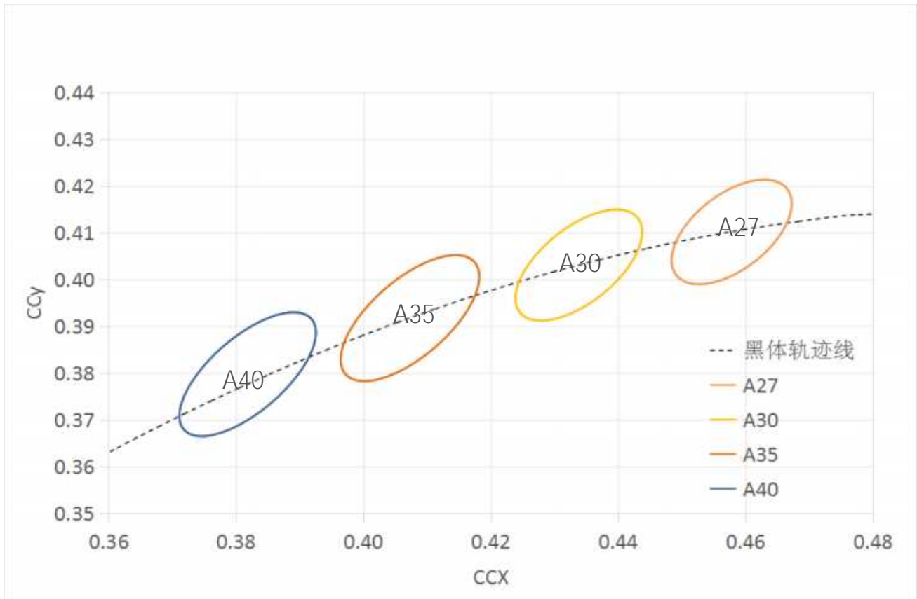
d) Chromaticity Region & Coordinates ( I_F = 700 \text{ mA} , T_s = 25^\circ\text{C} )
